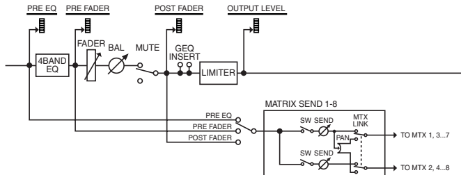
MATRIX SENDS (AUX 1-16, MAIN L/R)
