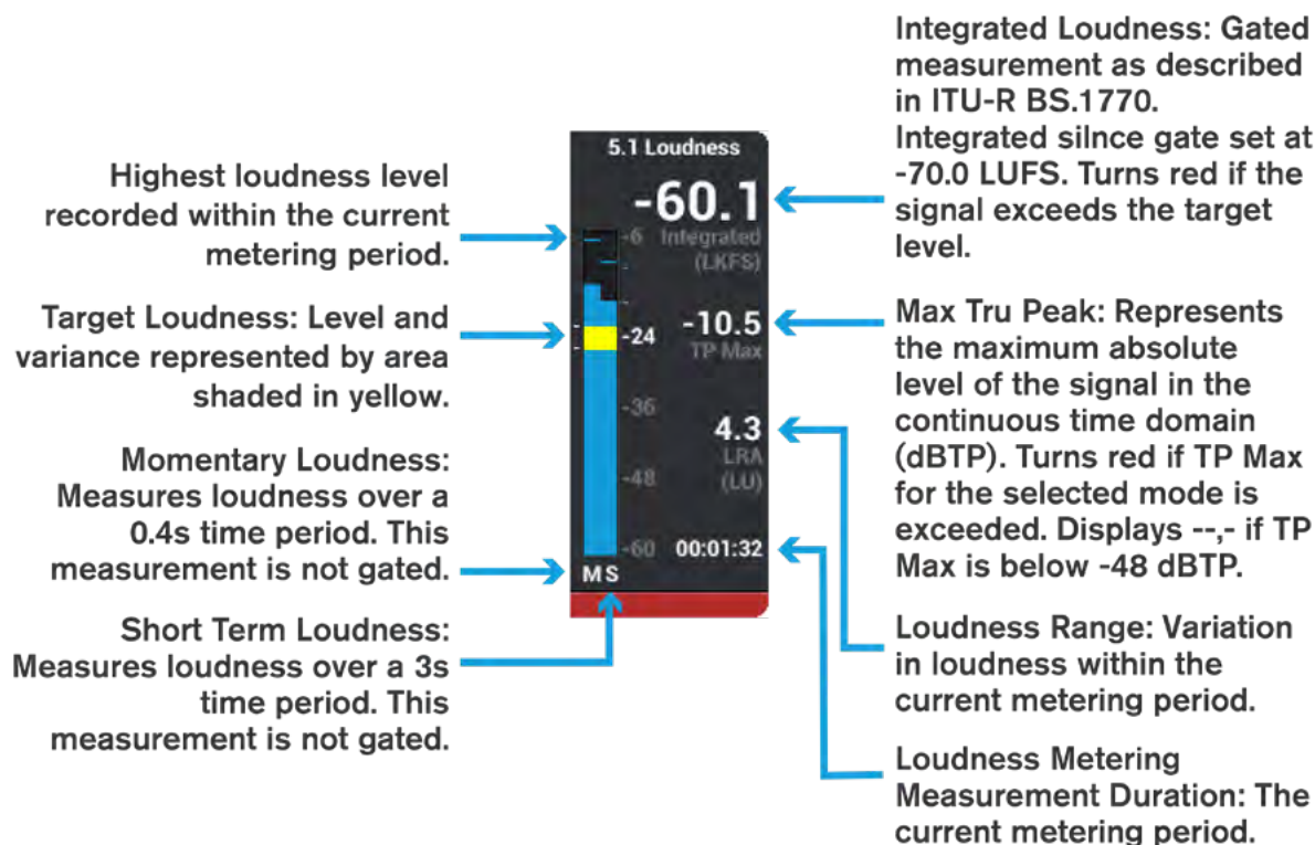
FIGURE 4 - LOUDNESS METERS
