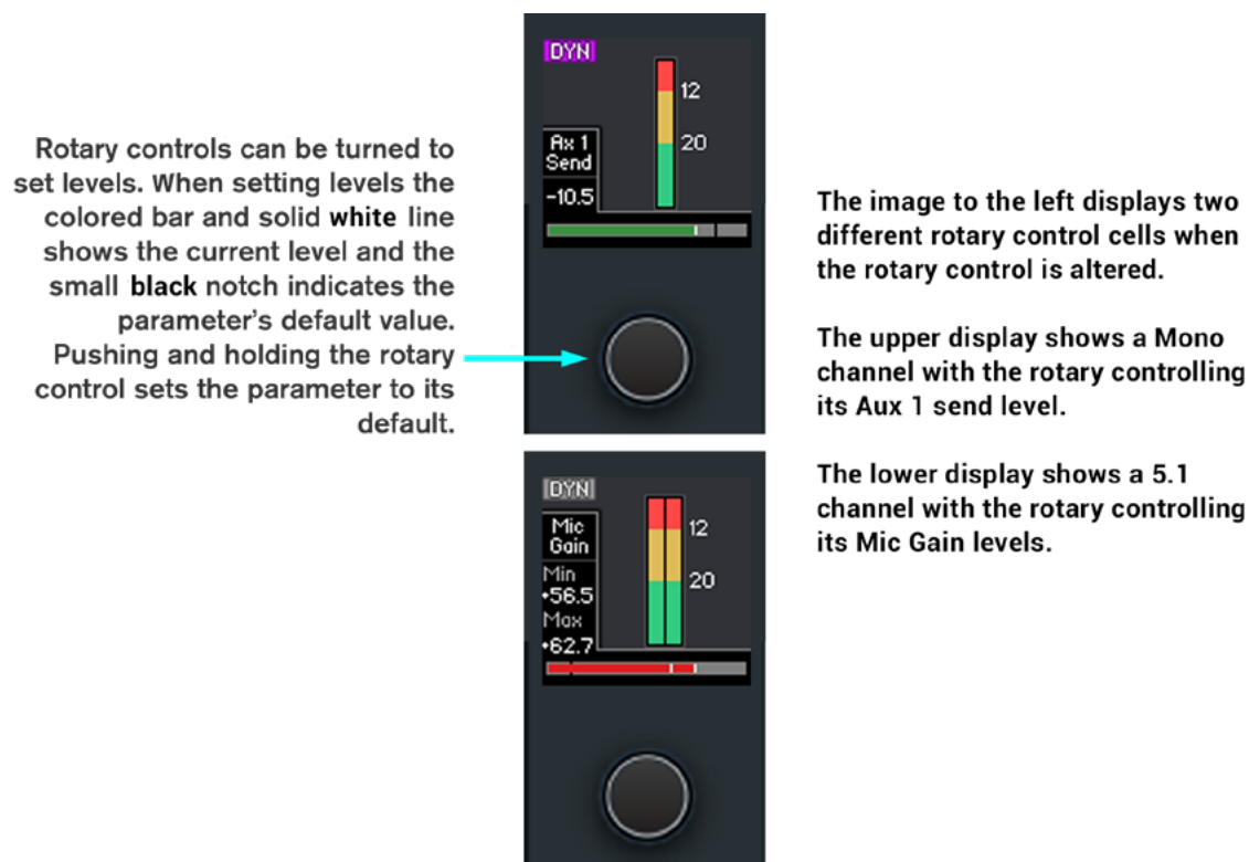
FIGURE 3 - CONTROL CELL
