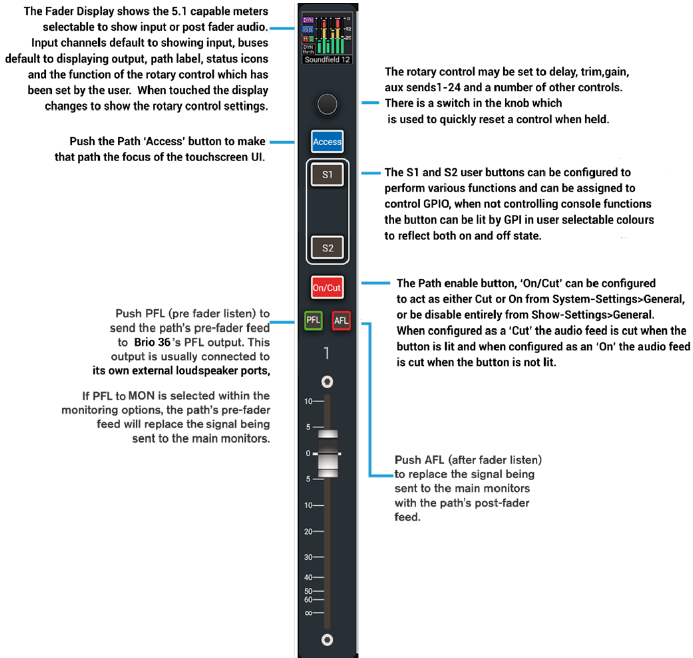
FIGURE 1 - FADER STRIP
